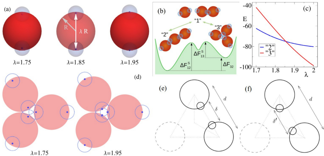
FIG. 1. (a) Example of three patchy particles: Two sticky spots of range \sigma (light blue spheres of radius \sigma with darker dot at their center) form a rigid body with a (red) repulsive core of radius R . The sticky spot centers are at distance \lambda R from each other. (b) Sketch of a possible free energy landscape for a trimer, i.e. a system with three patchy particles/micellar units. (c) Ground-state energy of linear-trimer (“2” state, blue) and branching-point (“3” state, red) configurations as a function of the branching parameter \lambda . (d) Sketch of a triple contact for \lambda = 1.75 (sticky spots farther than the interaction range \sigma ) and for \lambda = 1.95 (sticky spots closer than \sigma ). (e) and (f): Geometrical details of the (planar) linear and branched configurations. The total potential energy of a strand is E_l = 2u_l due to a full overlap of the sticky spots while, in a branching point, the same quantity is E_b = 3u_b with a bond energy |u_b| < |u_l| which tends to u_l only when \lambda is sufficiently large.
