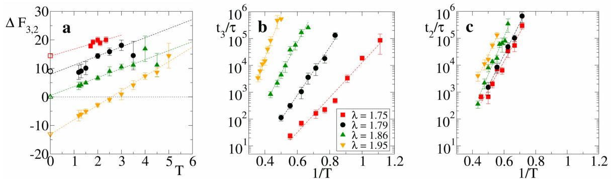
FIG. 3. Thermodynamic and kinetic properties of a trimer. (a) Free energy difference \Delta F_{3,2} vs. temperature T for \lambda = 1.75, 1.79, 1.86 and 1.95 . For the same values, -\Delta S_{32} = 2.4, 3.2, 3.2 and 5.1 from linear fits, see dashed lines. Open symbols reported on the vertical axis correspond to the energy difference from Fig. 1(c), at T = 0 . (b) Average scission time t_3 for a trimer initially arranged in the configuration “3” and (c) average scission time t_2 for a strand “2”, as a function of the inverse temperature 1/T . Dashed lines are Arrhenius fits of \Delta E_{13}^S and \Delta E_{12}^S . In all panels different symbols refer to different values of the branching parameter \lambda (see legend in panel (b))
