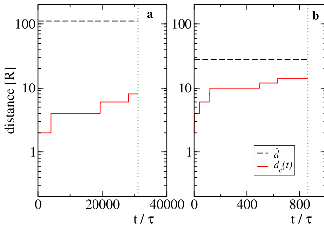
FIG. 9. Evolution of the maximal cluster size d_c(t) (red solid lines) for N = 25 (panel (a)) and N = 1600 (panel (b)). Black dashed horizontal lines indicate the values of the typical particle distance \bar{d} while green vertical lines identify the time at which f_0 reaches the threshold value f^* .
