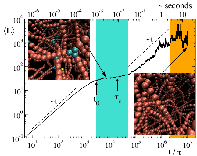
FIG. 4. Evolution of the average strand length \langle L \rangle for a system of N = 6000 particles with \lambda = 1.75 , and T = 1 (thick black curve). The cyan band marks the metastable regime with excess of branches (see an example in the upper inset) while the orange band identifies the regime of thermodynamic equilibrium (lower inset). Vertical arrows indicate the condensation time scale t_0 \simeq 3 \times 10^3\tau \approx 1 ms and the typical time \tau_s \simeq 2 \times 10^4\tau of network rearrangements. In the two configurations of the network, units with k = 1, 2, 3 contacts are drawn, respectively, in yellow, red and cyan.
