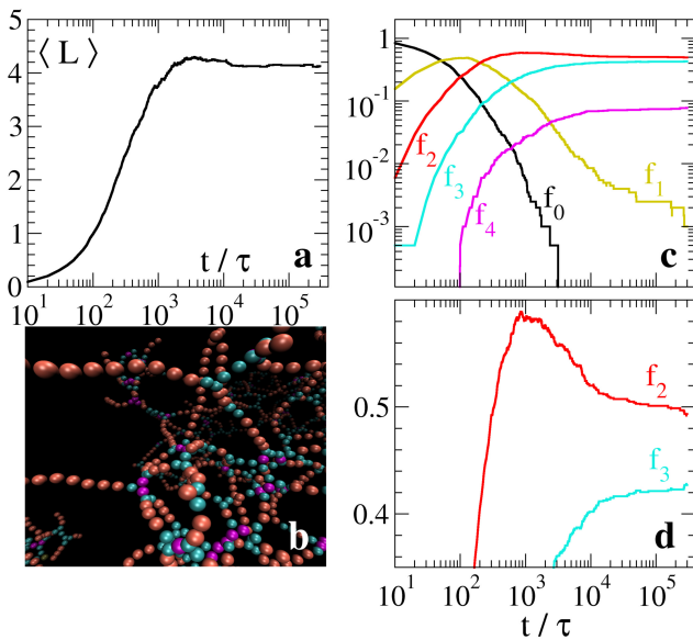
FIG. 6. Relaxation dynamics of a system with N = 2000 particles and \lambda = 2 for T = 1 . (a) Average strand length \langle L \rangle . (b) Final configuration of the network: gold, red, cyan, and magenta beads identify, respectively, units with k = 1, 2, 3, 4 contacts. (c) Evolution of the fraction f_k of units with k -contacts in log-log scale and (d) in linear-log scale.
