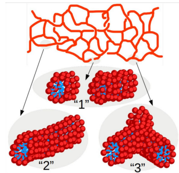
FIG. 2. Sketch of a wormlike micellar network and of selected portions where each surfactant is depicted as a hydrophilic (red) head and a hydrophobic (blue) tail. The numbering of the network portions follows that of the corresponding patchy particle states of Fig. 1(b).
