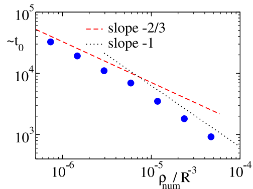
FIG. 7. Time scale of the network condensation as a function of the particle density. The straight lines indicate the scalings expected at low and high densities. Data refer to system sizes N = 25, 50, 100, 200, 400, 800, 1600 , T = 1 and \lambda = 1.8 . Particles are evolved in a cubic box with side equal to 324R and periodic boundary conditions.
