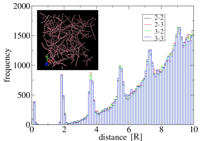
FIG. 8. Distribution of distances between sticky spots for a system of N = 2000 particles with \lambda = 1.75 , A = 40\epsilon and \sigma = 0.4R . Particles are prepared in a homogeneous state and evolved at T = 1 according to Eq. (A4) in a cubic box with side equal to 54R and periodic boundary conditions. The histogram is representative of the configuration obtained at t = 10^5\tau , see the inset. Black, red, green and blue bars refer respectively to the combination of indices (\alpha, \beta) = \{(2, 2), (2, 3), (3, 2), (3, 3)\} in the set of distances d_{i\alpha}^{j\beta} for i, j = 1, \dots, N . Their distributions overlap very well, as expected from symmetry reasons. Multiple peaks above the gap region derive from the regular spacing of particles in the strands.
