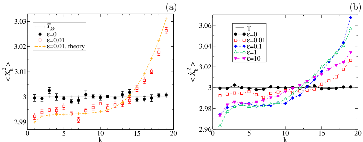
Figure 3. Kinetic energy of the normal modes for a chain of N = 20 unit masses coupled via quadratic-quartic potential (harmonic constant \kappa = 1 , quartic \epsilon = 0, \dots, 10 ) and immersed in heat baths characterised by the (global) friction constant \gamma = 0.1 and the local temperatures T_i , which grow linearly with i from T_0 = 1 to T_{N-1} = 5 (in natural dimensionless units). (a) Comparison between the analytic expansion (37) (+) and the numerically estimated \langle \dot{X}_k^2 \rangle ( \square ) obtained by integration of the oscillators' stochastic dynamics. (b) Numerically estimated mode kinetic energies also for strongly anharmonic chains. Errors are of the order of symbol sizes.
