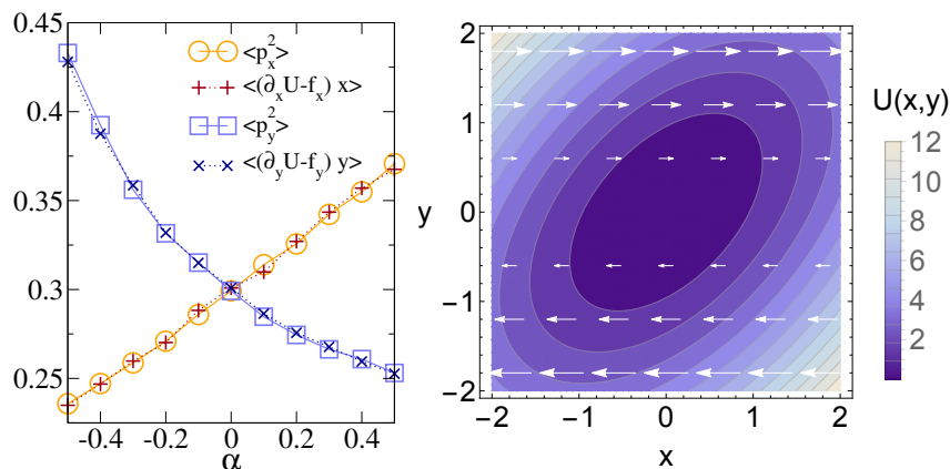
Figure 1. The mesoscopic virial theorem (MVE) as a function of the shear force strength \alpha , for each degree of freedom of a particle moving in two dimensions subject to the potential and forces sketched on the right for \alpha > 0 . The temperature is T = 0.3 and the damping constant is \gamma = 0.2 , in natural units.
