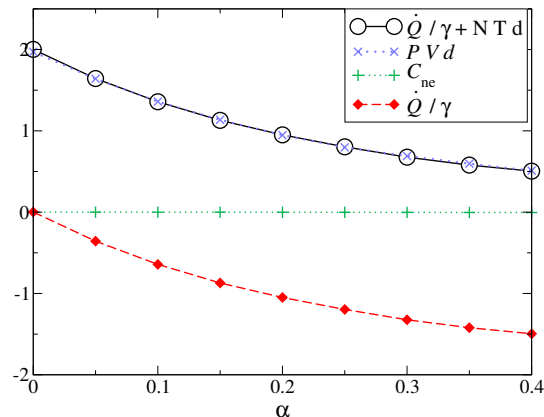
Figure 2. Contributions in Eq. (18) for a spatially confined Langevin particle at temperature T = 1 (natural dimensionless units), subjected to an extra dry friction \mathbf{f} = -\alpha \mathbf{v}/|\mathbf{v}| . The negative sign of the mean heat flow into the reservoir, \dot{Q} < 0 , is consistent with a positive heat absorbed on average by the system when solid friction dissipates energy ( \alpha > 0 ).
