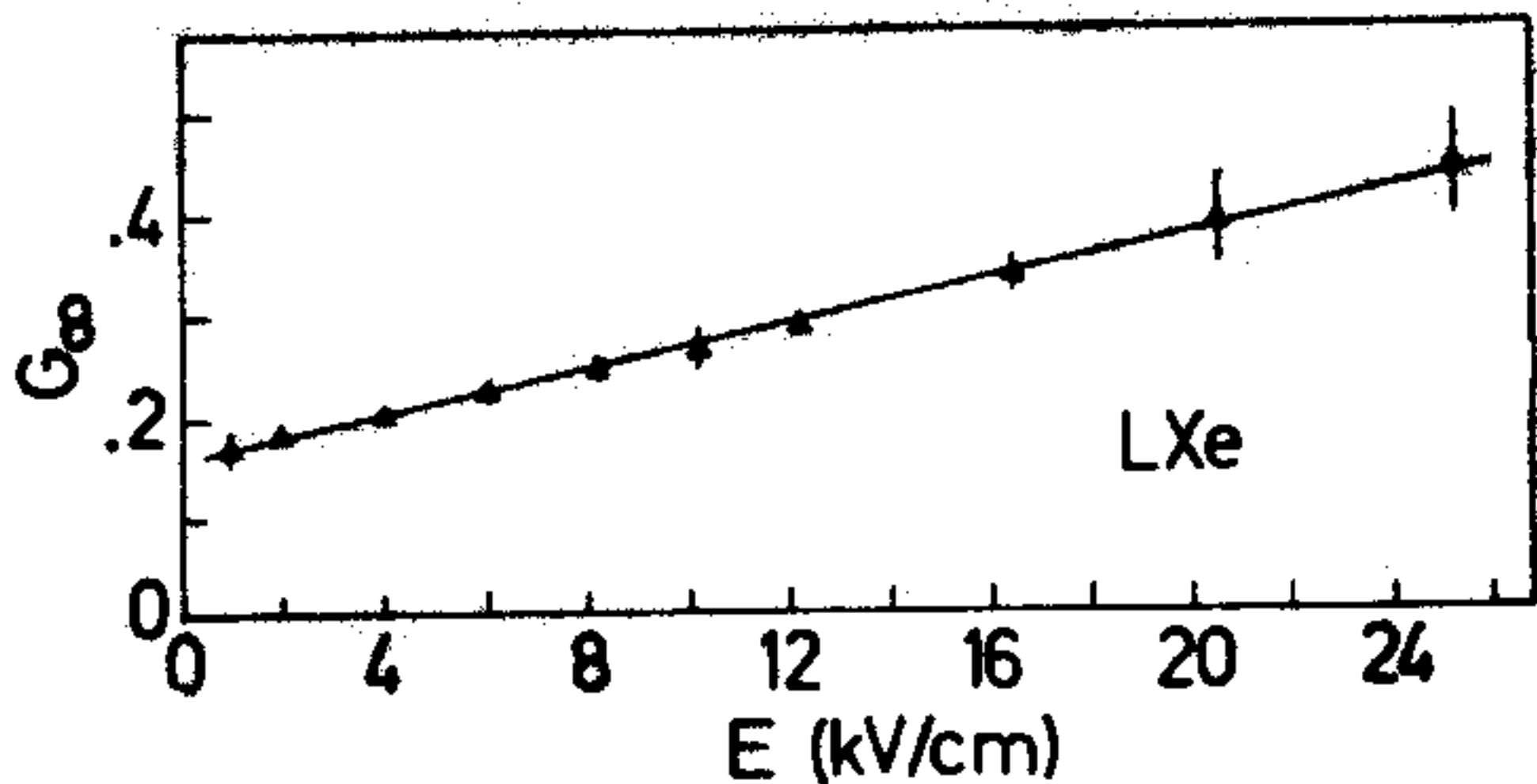
Fig. 9. Liquid xenon free carrier yield for 5.4 MeV alpha-particles as obtained in the present investigation.
