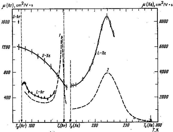
FIG. 3. Temperature dependence of electron mobility in the limit of zero field; L —liquid, S —crystal. Dashed lines—results of earlier work: 1—Ref. 3, 2—Ref. 5.
