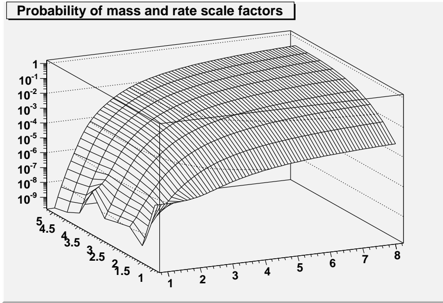
Figure 8: Probability to observe a D_0 -like signal in data containing a CDF-like one, as a function of the scale factor k applied on the systematic uncertainty affecting the D_0 mass measurement (running from 1.0 to 8.0 on the x -axis), and as a function of the scale factor \gamma applied on the rate of \Omega_b candidates expected in the D_0 histogram by assuming the CDF measured rate (running from 1.0 to 5.0 on the y axis). See the text for caveats and details.
