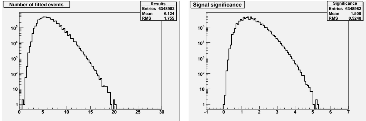
Figure 3: left: Number of signal events in the Gaussian (of width equal to the D0 mass resolution) fit in pseudo-histograms containing 79 events. Right: Significance of D0 -like pseudoexperiments, computed using delta-log-likelihood values. The wiggling of the distributions reflects the discreteness of the distributions created by the pseudoexperiments.
