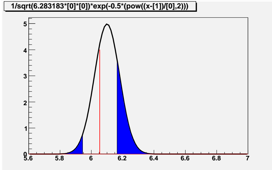
Figure 6: Graphical explanation of the method used to compute the probability of a mass measurement at least as distant from the CDF measurement as the one obtained by D0. The red line is at M_{CDF} = 6054.4 \text{ MeV} ; the Gaussian has a mean equal to the fit mass of a pseudoexperiment finding a signal exceeding 18.4 events, and a width equal to the one expected if a large scale factor k (exaggerated for display purpose) is hypothesized for the systematical uncertainty in the D0 mass measurement. By integrating the blue area of the Gaussian, we obtain an estimate of the probability that a value as discrepant as the D0 one was observed.
