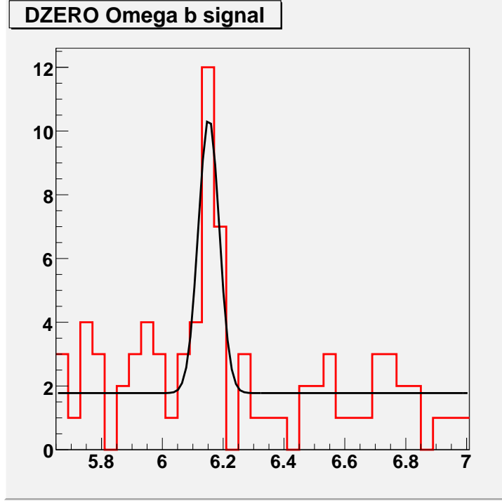
Figure 2: Result of a binned likelihood fit to the mass histogram of the 79 D0 \Omega_b candidates. The fit returns a signal of 18.4 events.
