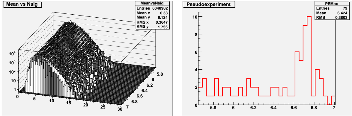
Figure 4: Left: number of fit events versus fit mass in the background-only pseudoexperiments mimicking the experimental data of D_0 . Right: the pseudo-histogram which mimics the largest signal in the set of over 6.3 millions.
