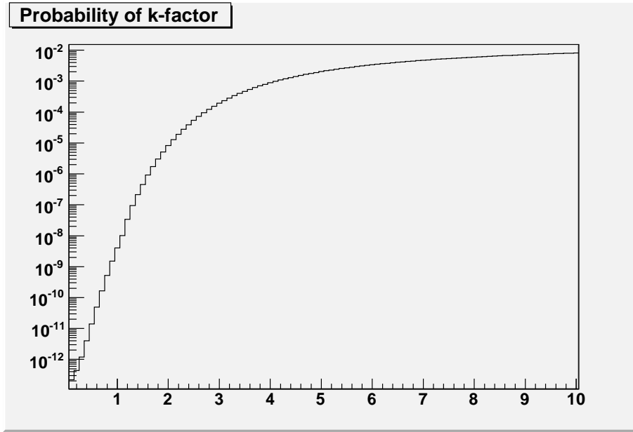
Figure 7: Probability to observe a D_0 -like signal in data containing a CDF-like one, as a function of the scale factor k applied on the systematic uncertainty affecting the D_0 mass measurement.
