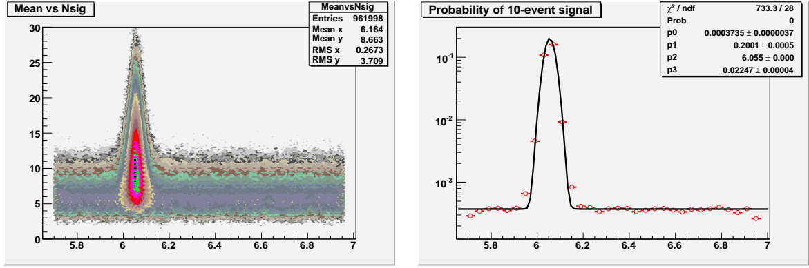
Figure 5: Results of 961,998 binned-likelihood fits to 79-event pseudo-histograms generated with a CDF-like \Omega_b signal of normalization chosen as explained in the text. Left: number of events returned by the fit as a function of the fit mass; right: relative fraction of pseudoexperiments returning a signal of N_{fit} > 10 events. Note the outlier bins above the fit line on each side of the Gaussian.
