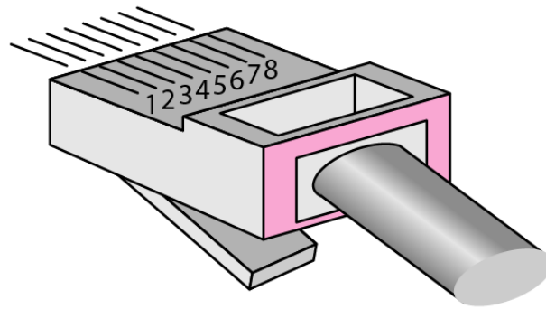
RJ-45 Male
